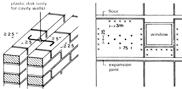
① Wire ties for external double leaf cavity walls ② Anchoring of the outer leaf → pp. 63-4
